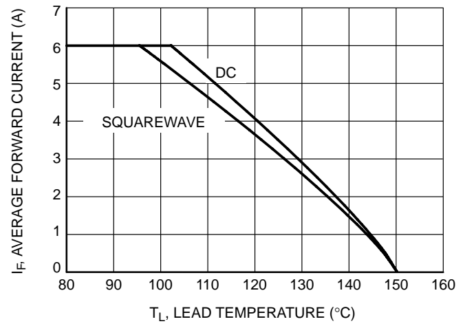
Figure 7. Derating Curve
