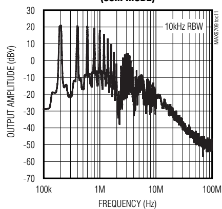
WIDEBAND OUTPUT SPECTRUM (SSM MODE)
