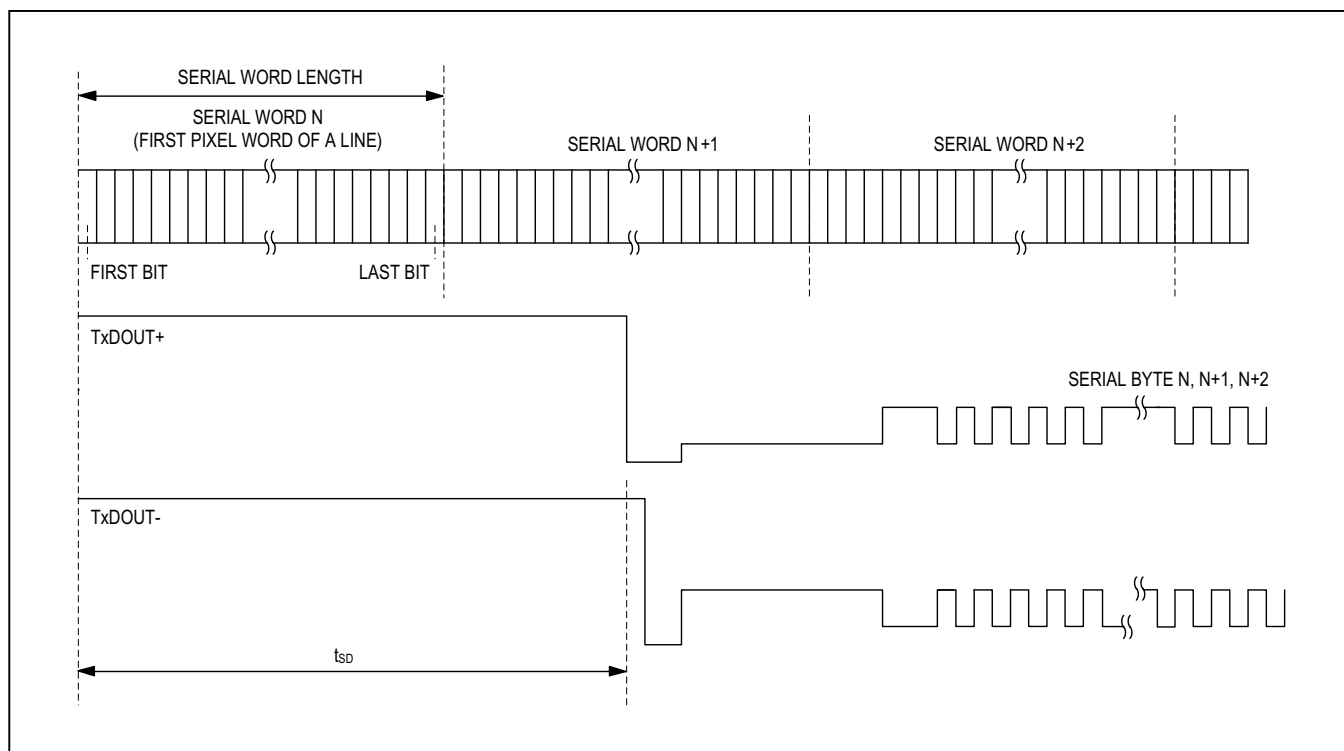
Figure 8. Deserializer Delay
