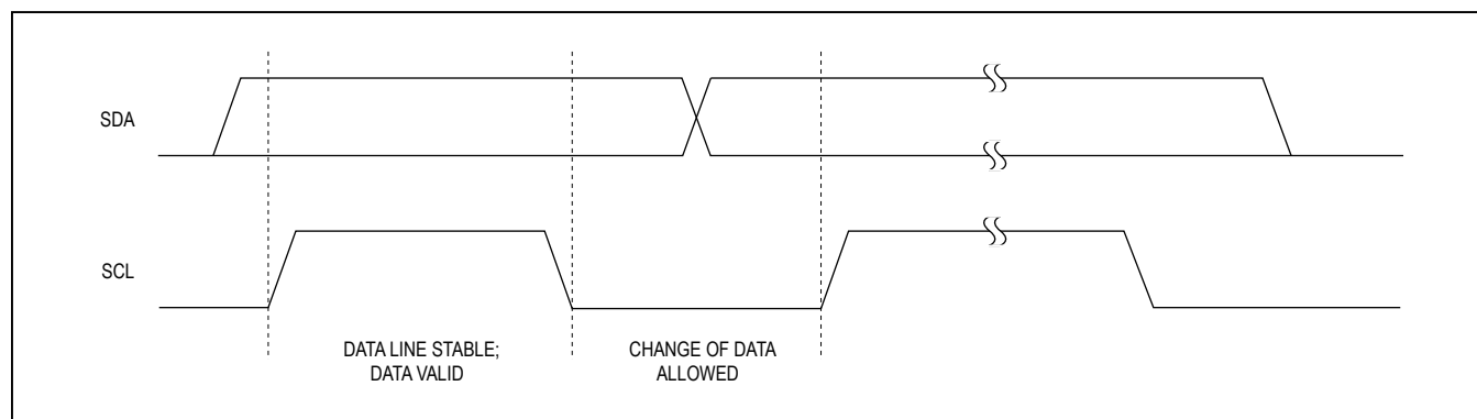
Figure 48. Bit Transfer
