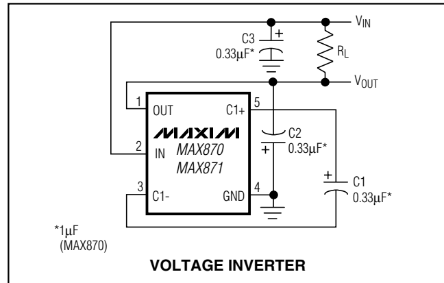
Figure 1. Test Circuit
