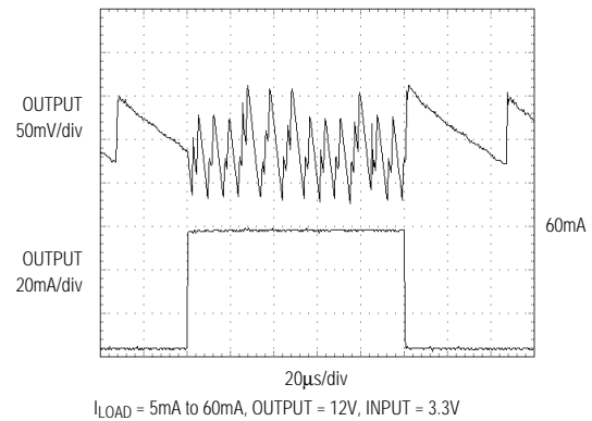
MAX607 LOAD-TRANSIENT RESPONSE
