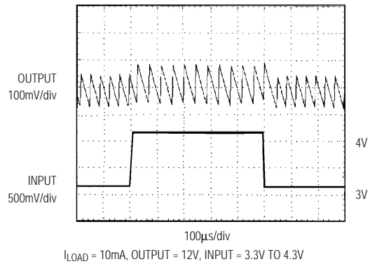
MAX607 LINE-TRANSIENT RESPONSE
