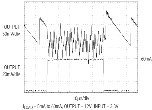
MAX606 LOAD-TRANSIENT RESPONSE
