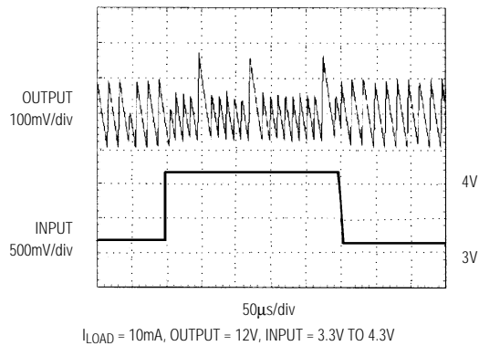
MAX606 LINE-TRANSIENT RESPONSE
