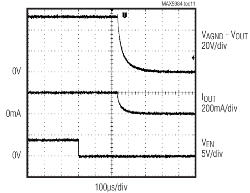
EN TO OUT TURN-OFF DELAY
