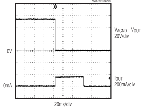
SHORT-CIRCUIT RESPONSE TIME
