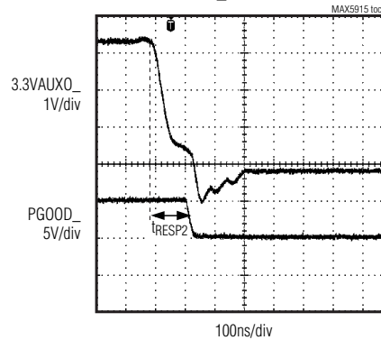
MAX5915A/MAX5916A 3.3VAUXO_ SHORT CIRCUIT
