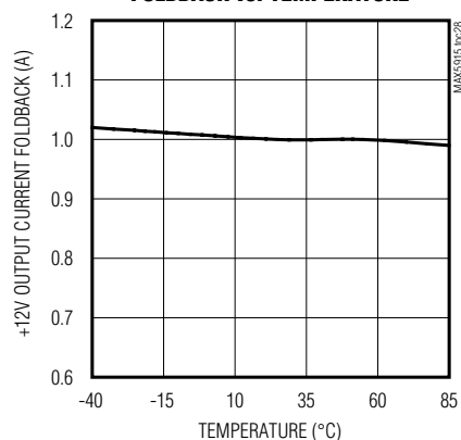
+12V OUTPUT CURRENT FOLDBACK vs. TEMPERATURE
