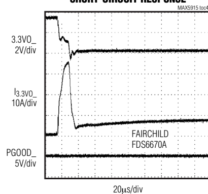
3.3VO_ IMMEDIATE SHORT-CIRCUIT RESPONSE
