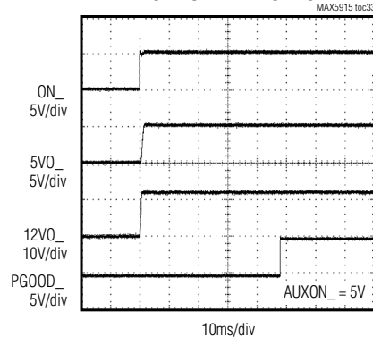
MAIN SUPPLY TURN-ON WAVEFORMS
