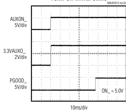
AUXILIARY SUPPLY TURN-ON WAVEFORMS
