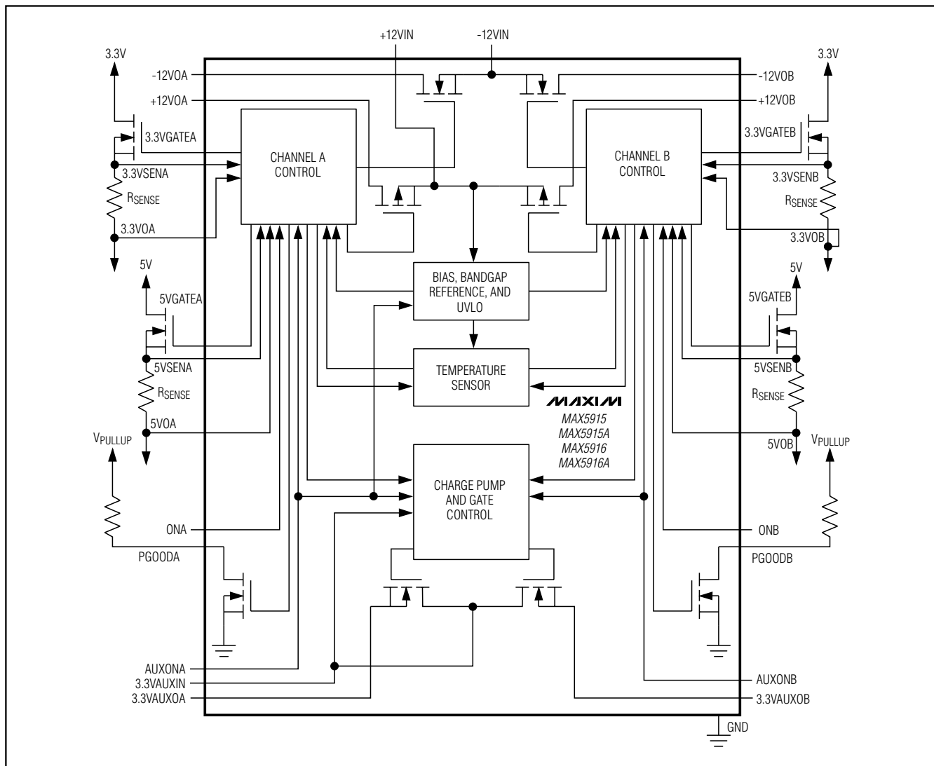
Functional Diagram
