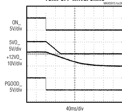
MAIN SUPPLY TURN-OFF WAVEFORMS
