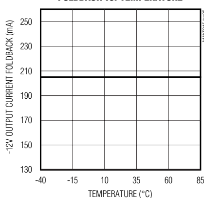
-12V OUTPUT CURRENT FOLDBACK vs. TEMPERATURE
