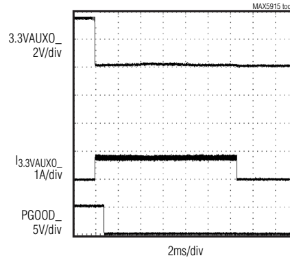
3.3VAUXO_ CURRENT FOLDBACK
