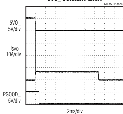
5VO_ CURRENT LIMIT
