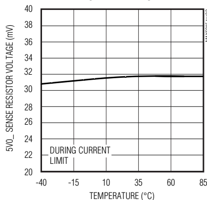
5V SENSE RESISTOR VOLTAGE vs. TEMPERATURE
