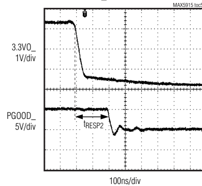
MAX5915A/MAX5916A 3.3VO_ SHORT CIRCUIT
