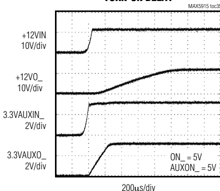
TURN-ON DELAY
