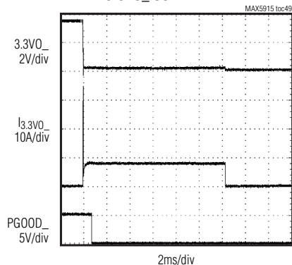
3.3VO_ CURRENT LIMIT
