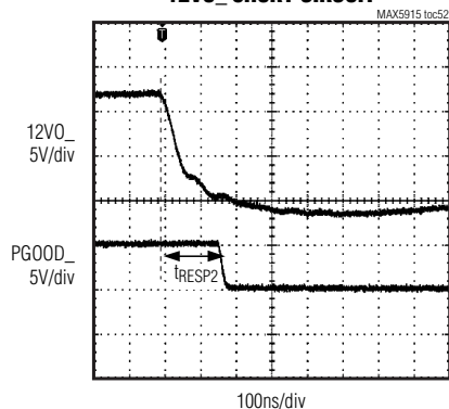
MAX5915A/MAX5916A 12VO_ SHORT CIRCUIT
