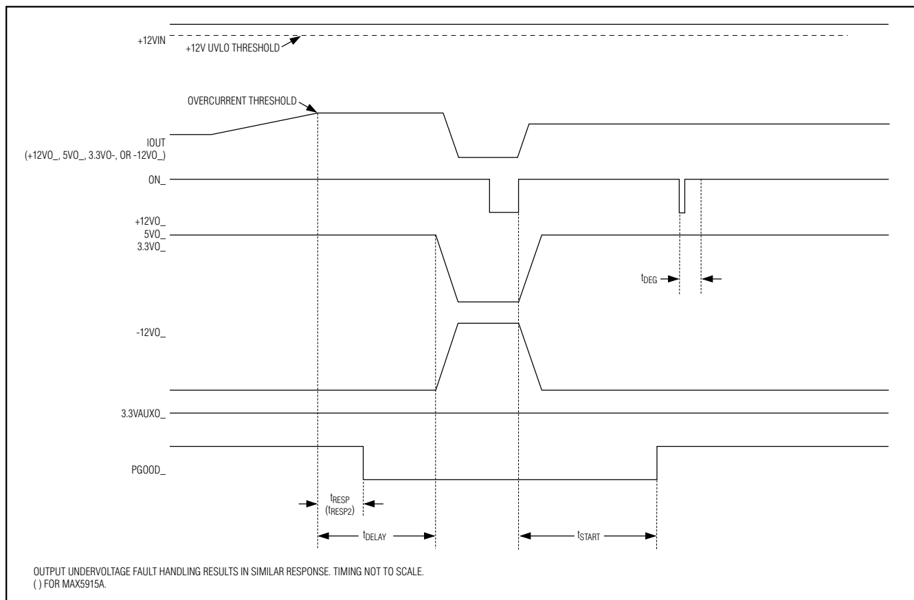
Figure 5. Main Outputs Overcurrent Fault Management in the MAX5915/MAX5915A
