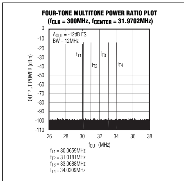
Figure 12. Four-Tone MTPR Test Results
