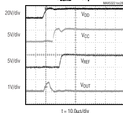
UNIPOLAR STARTUP RESPONSE, C_{LOAD} = 230\text{pF}
