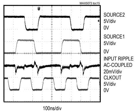
OUT-OF-PHASE OPERATION
