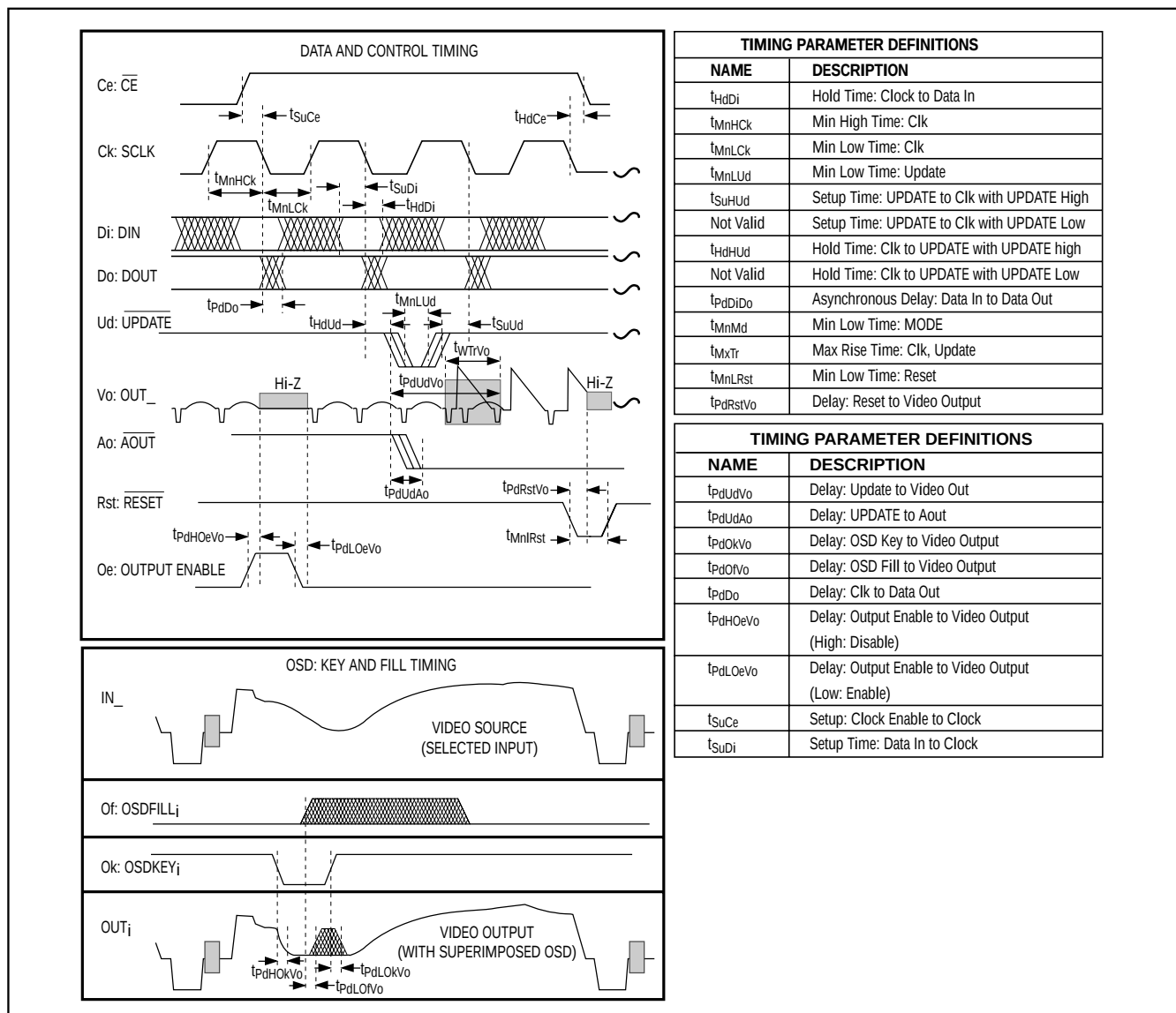
Figure 1. Timing Diagram
