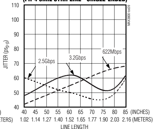
EQUALIZER RESIDUAL JITTER vs. LINE LENGTH (FR-4 6MIL STRIPLINE - SINGLE-ENDED)
