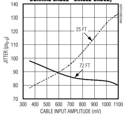
EQUALIZER RESIDUAL JITTER vs. CABLE INPUT AMPLITUDE (RG179B 75Ω COAXIAL CABLE - SINGLE-ENDED)
