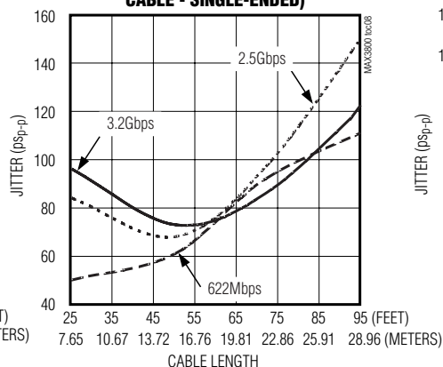
EQUALIZER RESIDUAL JITTER vs. CABLE LENGTH (RG179B 75Ω COAXIAL CABLE - SINGLE-ENDED)
