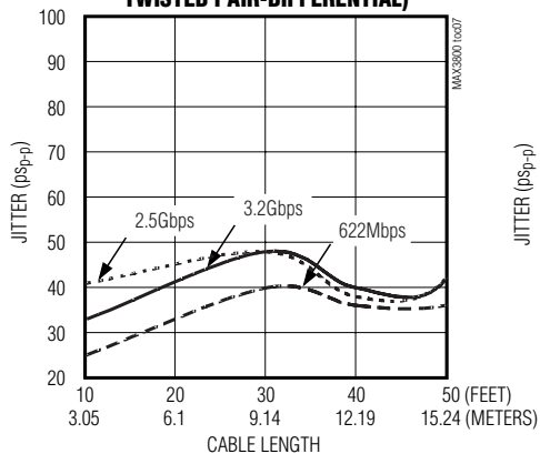
EQUALIZER RESIDUAL JITTER vs. CABLE LENGTH (MADISON #13887 SHIELDED TWISTED PAIR-DIFFERENTIAL)
