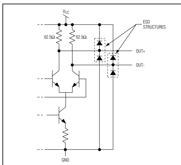
Figure 3. CML Output Equivalent Circuit
