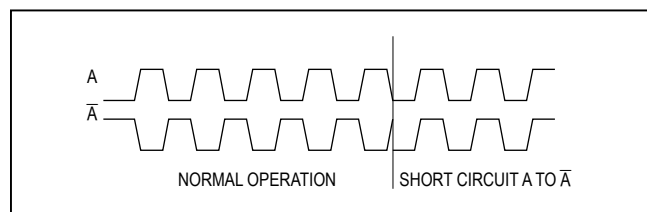
Figure 8. Short-Circuit Detection
