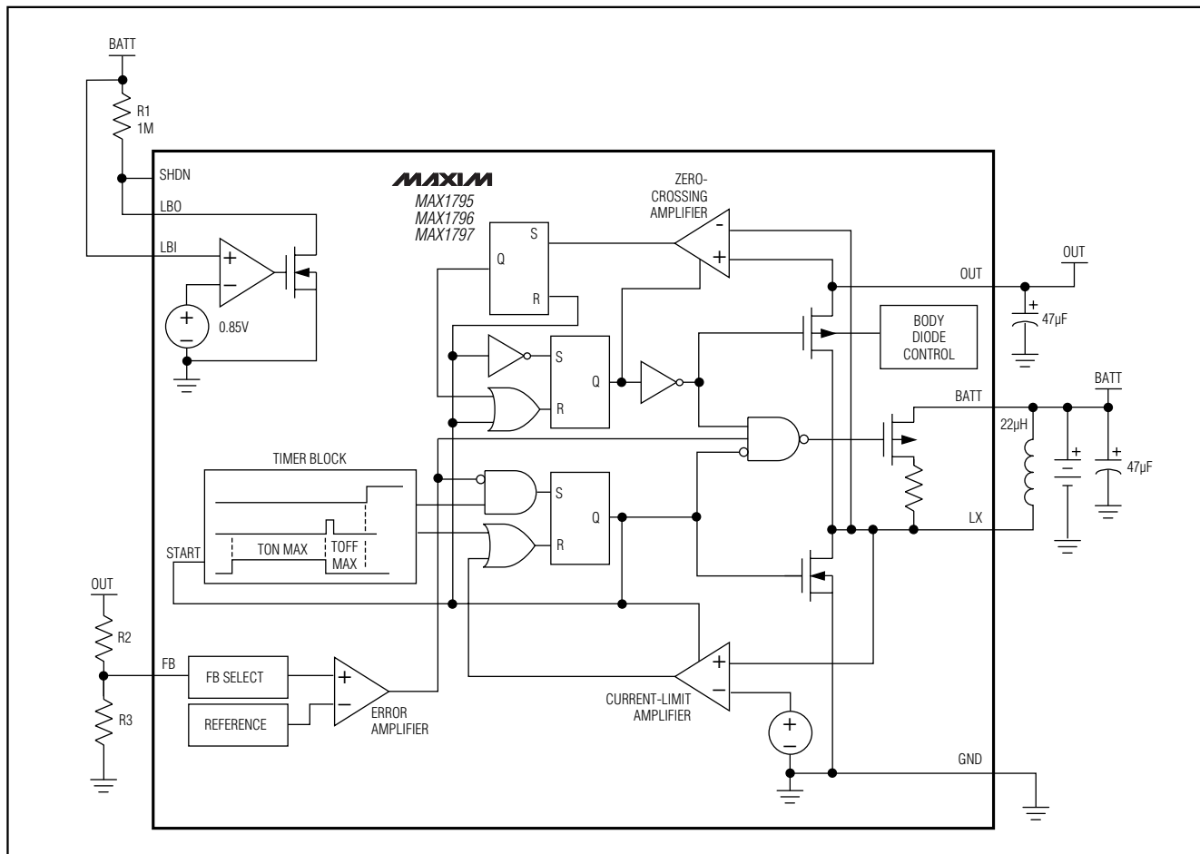
Figure 2. Functional Diagram
