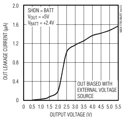
OUT LEAKAGE CURRENT vs. OUTPUT VOLTAGE
