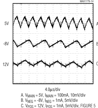
RIPPLE WAVEFORMS
