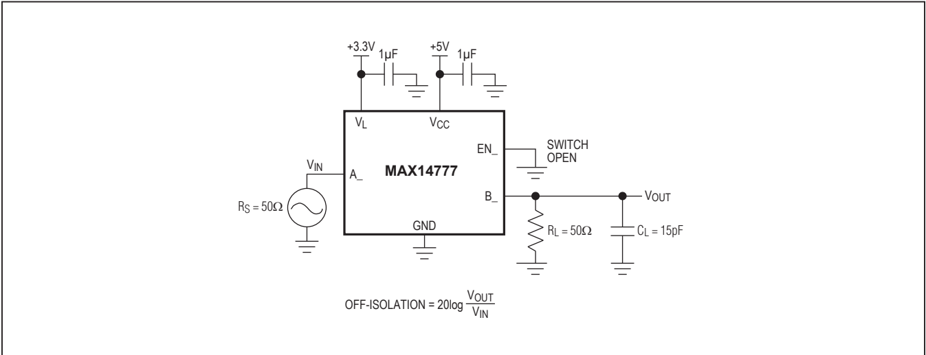
Figure 4. Off-Isolation
