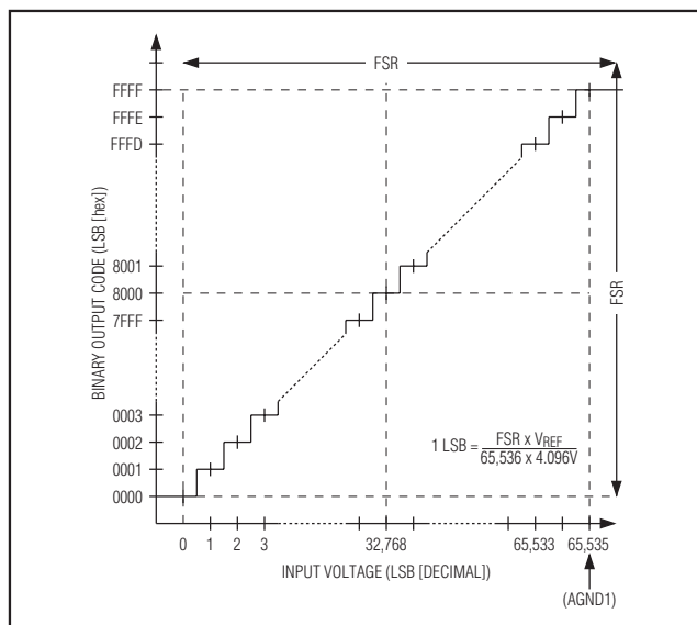
Figure 13. Ideal Unipolar Transfer Function, Single-Ended Input, -FSR to 0
