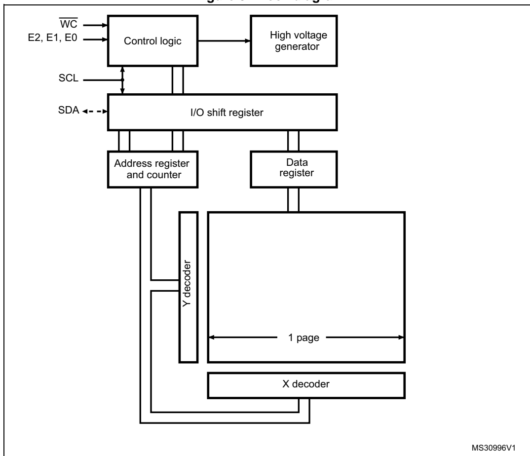
Figure 3. Block diagram
