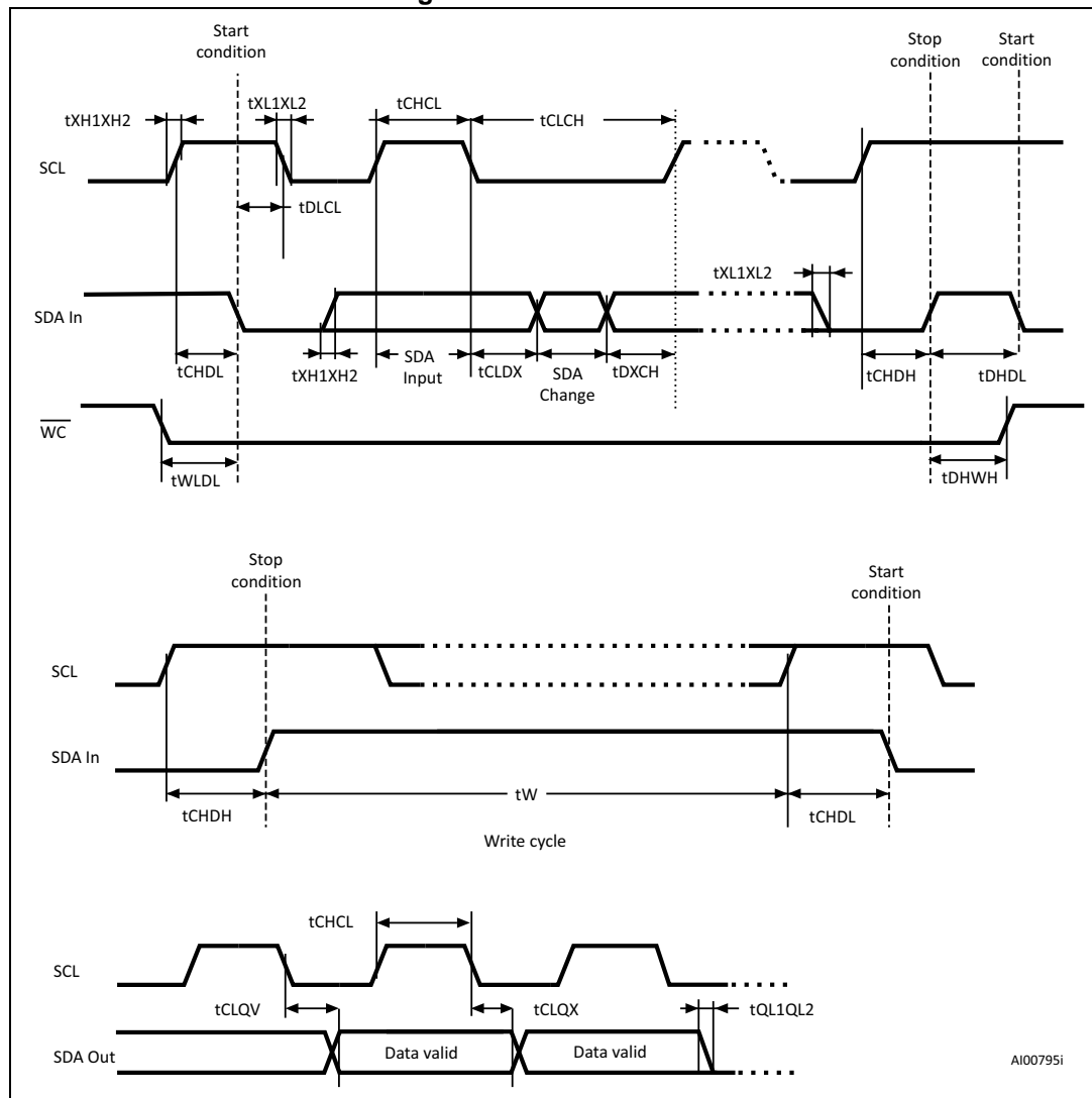
Figure 11. AC waveforms
