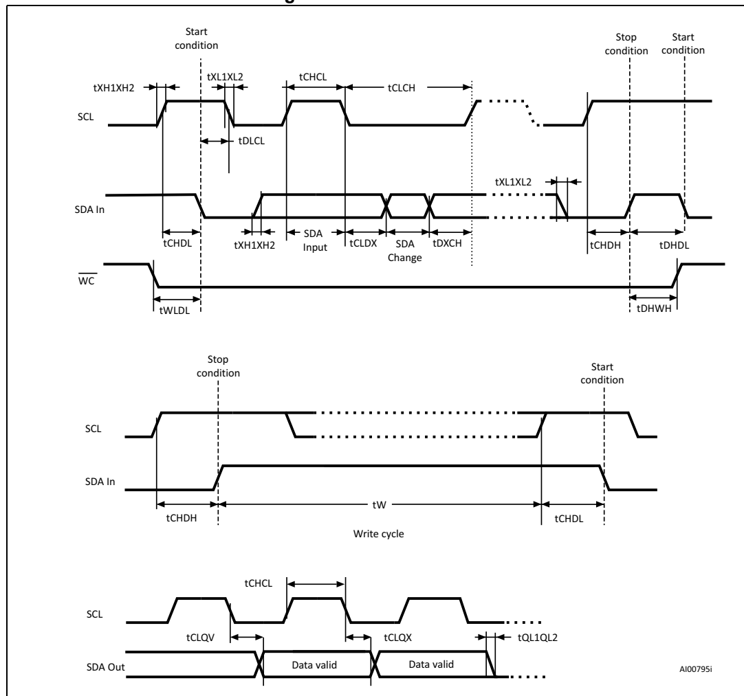
Figure 11. AC waveforms
