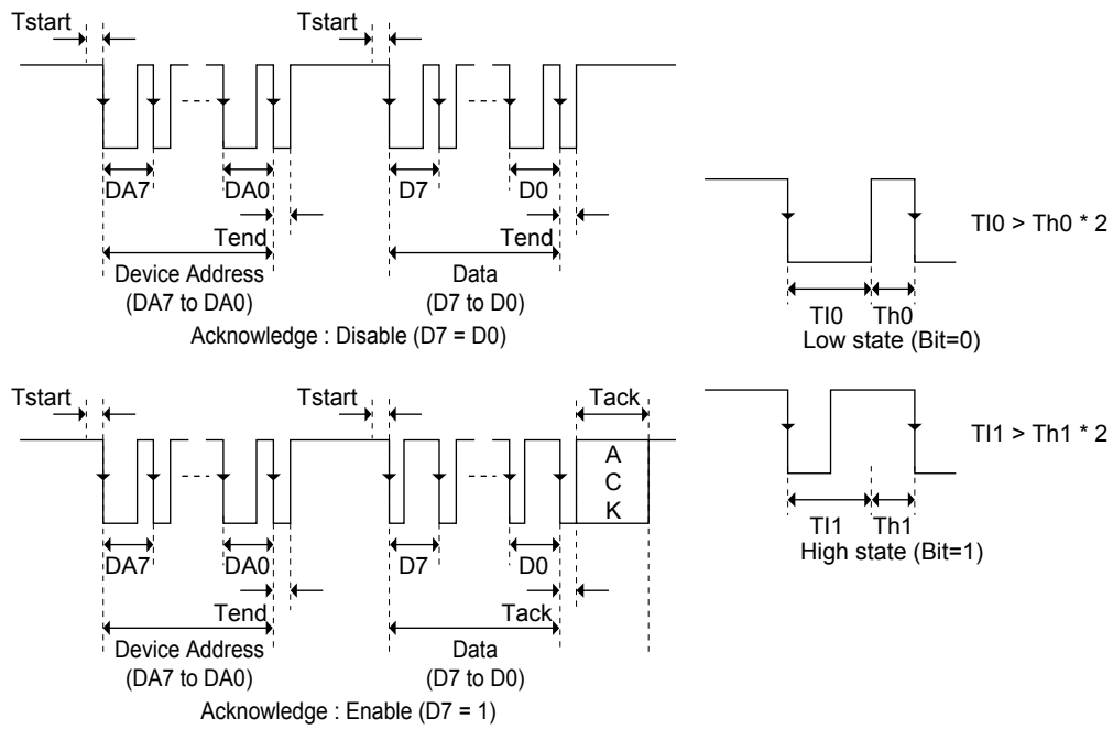
Fig6.Bit detection Diagram
