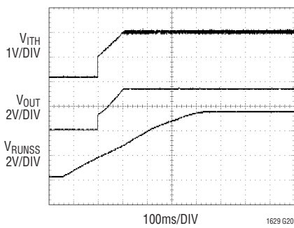
Soft-Start Up (Figure 12)
