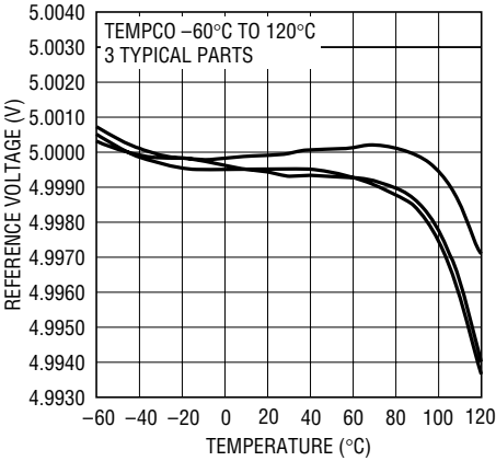
5V Reference Voltage vs Temperature
