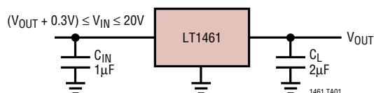
Basic Connection
