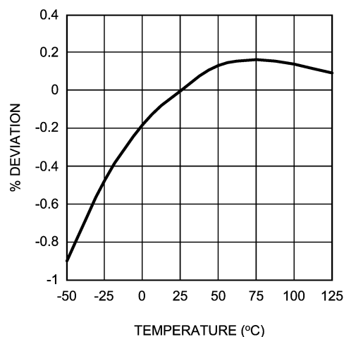
V_{OUT} vs Temperature (3.3V)
