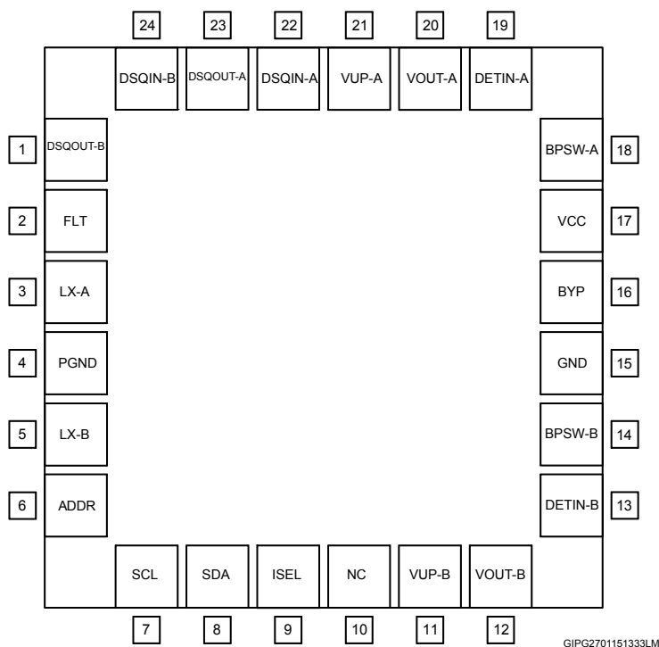
Figure 5. Pin connections (top view)
