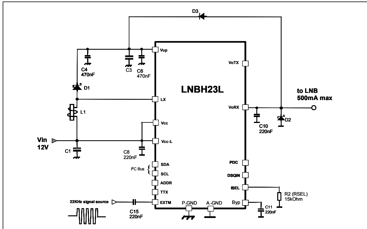
Figure 5. DiSEqC 1.x using external 22 kHz tone generator source through EXT pin
