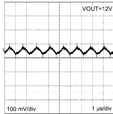
Output Ripple
