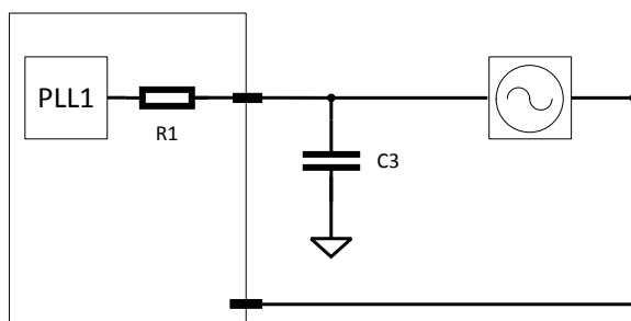
Figure 37. 3 rd Order Loop Filter
