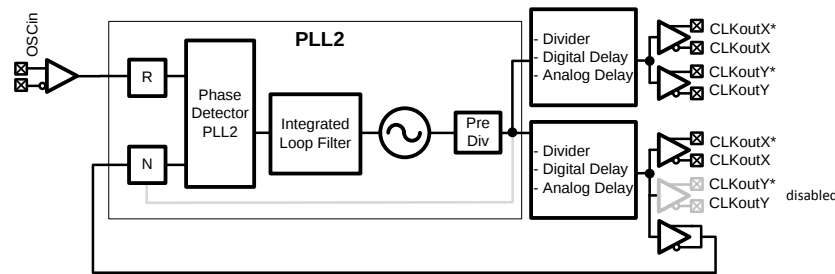
Figure 48. Low Skew Mode
