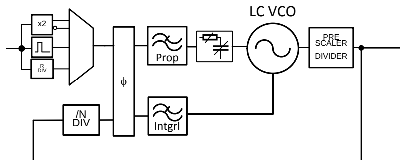
Figure 39. PLL2 Blockdiagram
