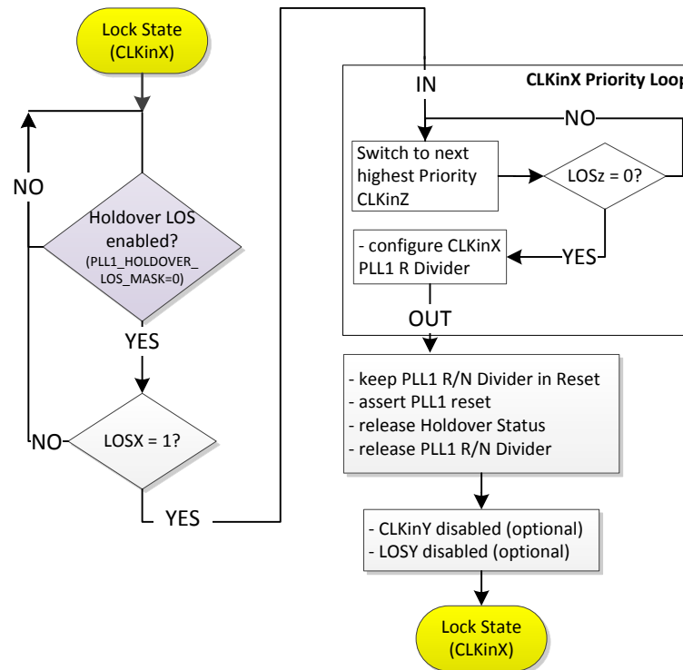
Figure 16. Input Clock Switching – Priority Loop
