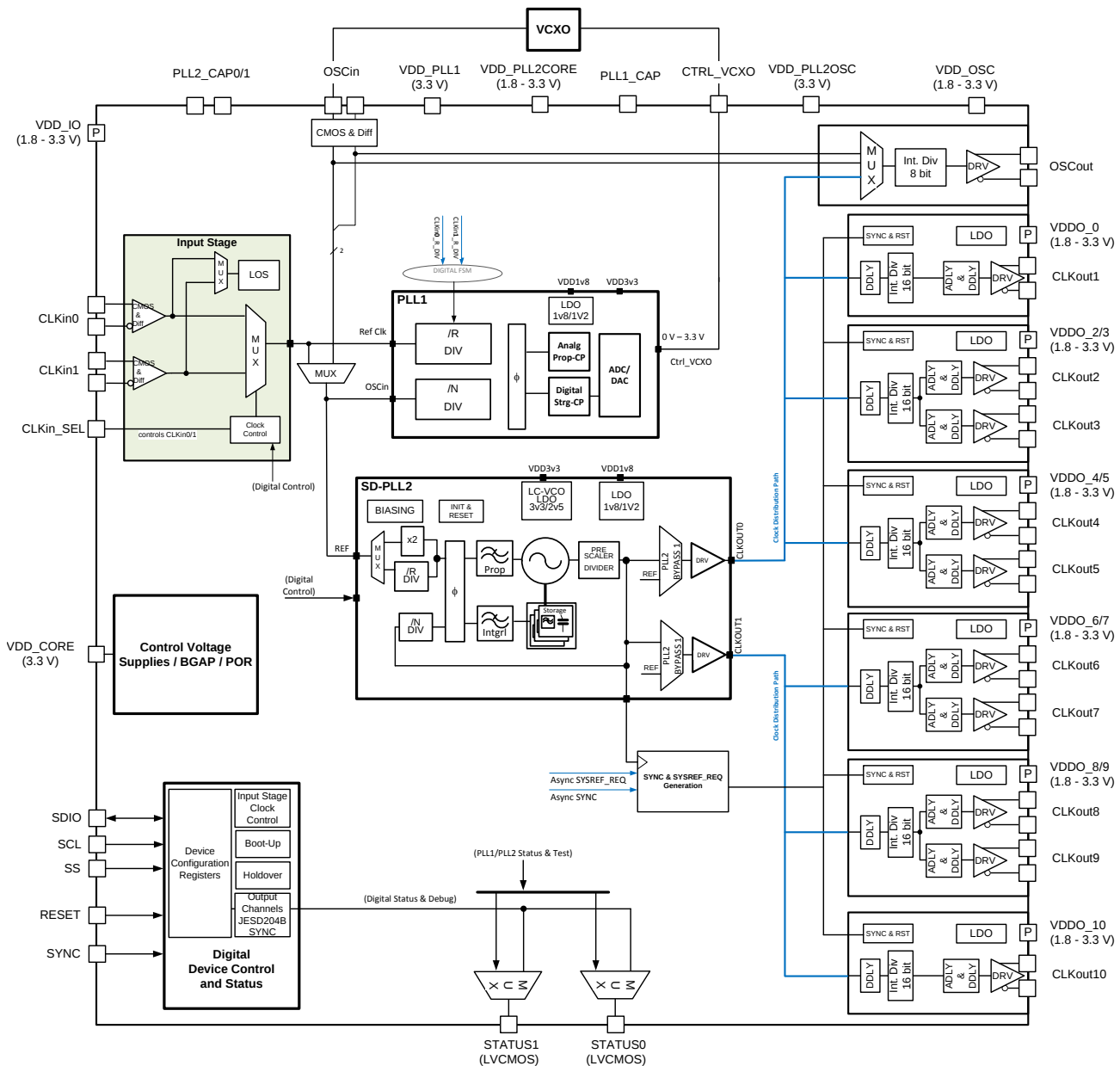
Figure 14. Detailed LMK04610 Block Diagram
