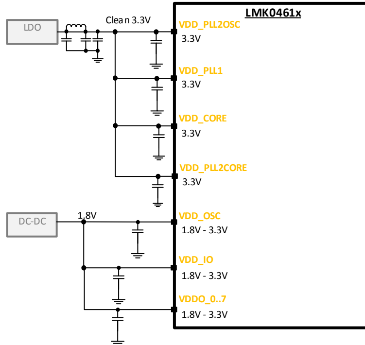
Figure 60. Recommended Power Supply Connection
