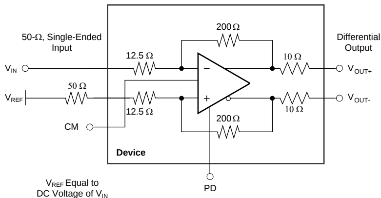
Figure 67. Active Balun
