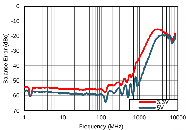
Figure 68. Balance Error
