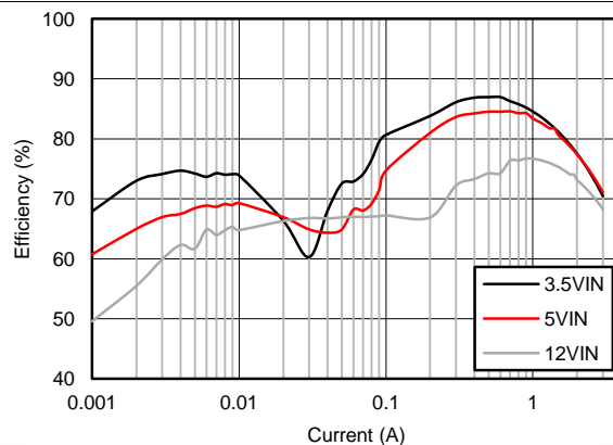
Figure 50. Efficiency
