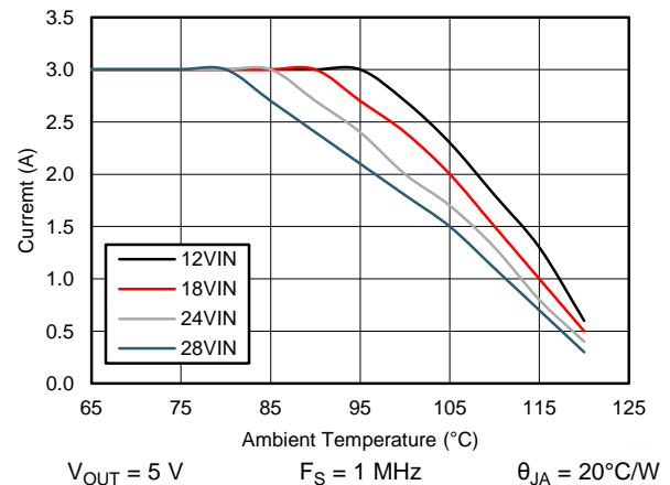
Figure 84. Derating Curve
