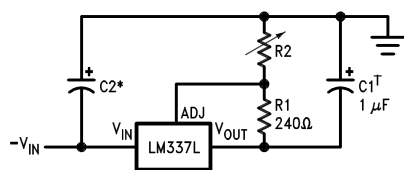
1.2V-25V Adjustable Regulator
