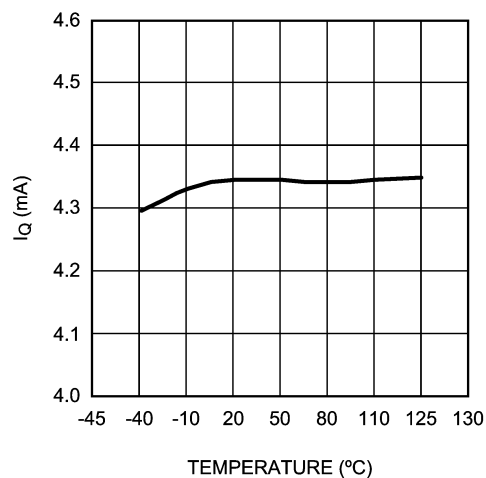
LM2831Z I_Q (Quiescent Current)
