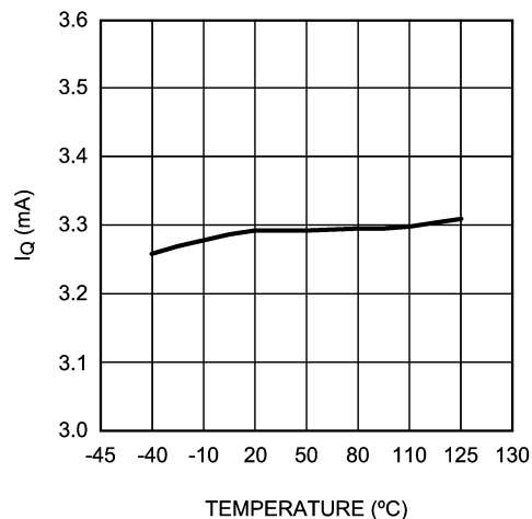
LM2831X I_Q (Quiescent Current)
