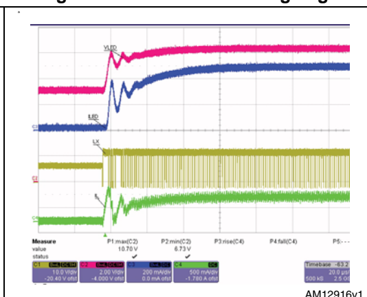
Figure 29. Hiccup current protection
