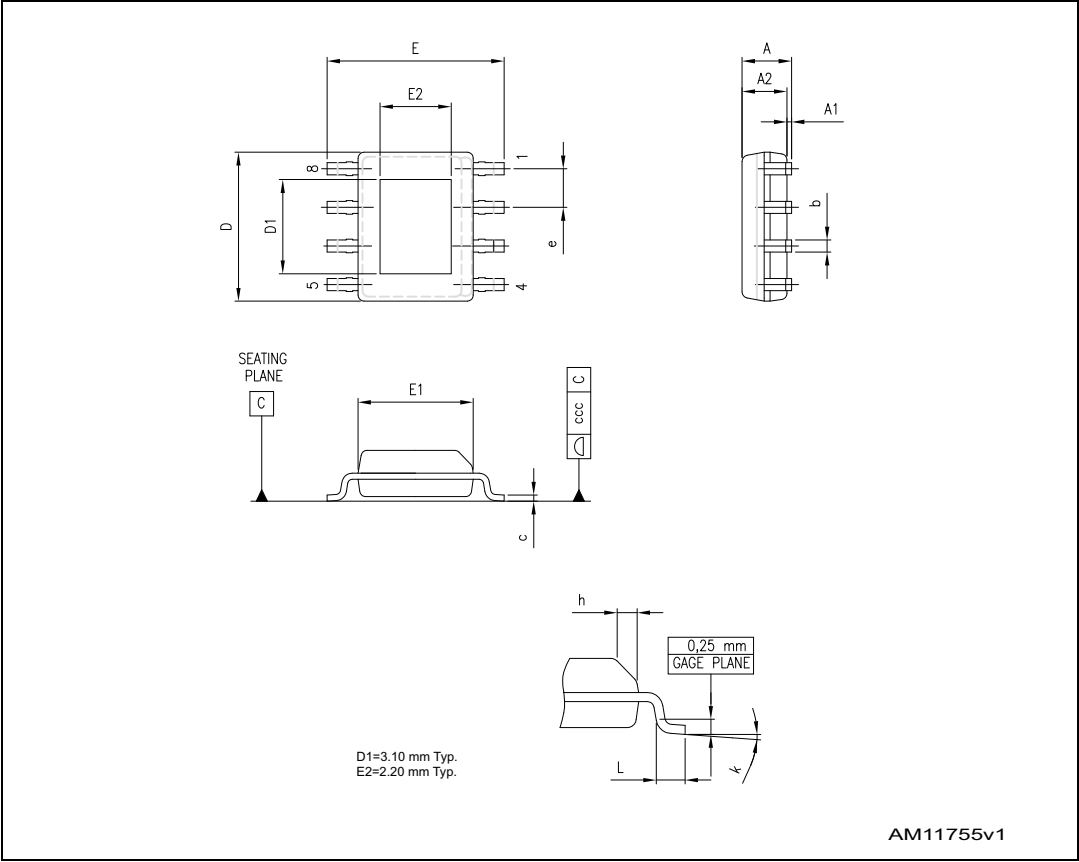
Figure 33. HSOP8 package dimensions
