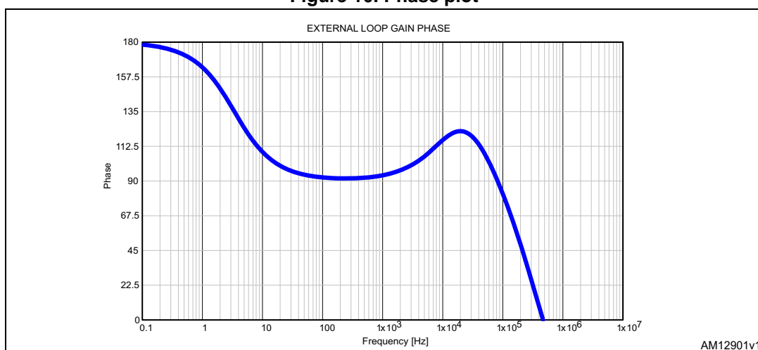
Figure 10. Phase plot
