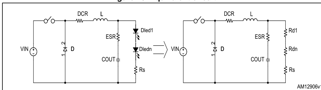
Figure 15. Equivalent circuit
