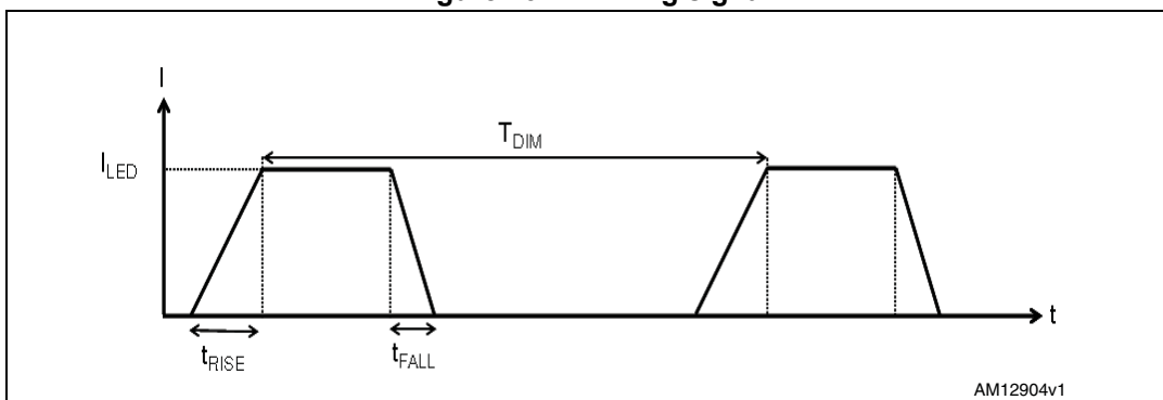
Figure 13. Dimming signal
