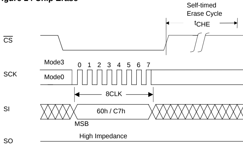
Figure 14 Chip Erase
