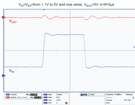
Figure 16. Line transient
