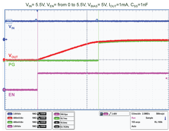
Figure 21. Turn-on time ( C_{SS} = 10 \text{ nF} )
