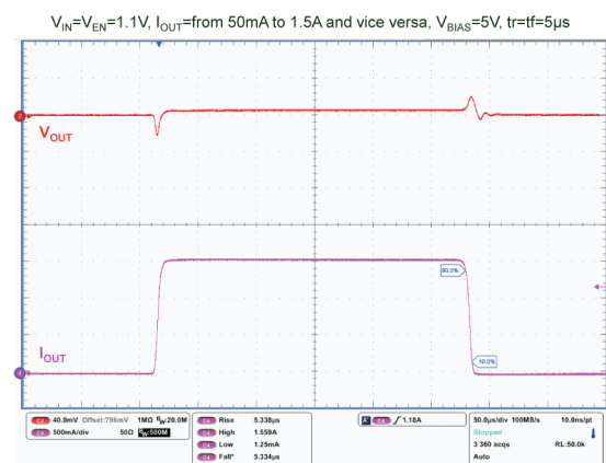
Figure 17. Load transient
