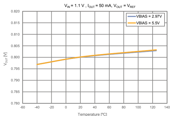
Figure 4. Output voltage vs. temperature and V_{BIAS} ( I_{OUT} = 50\text{ mA} )
