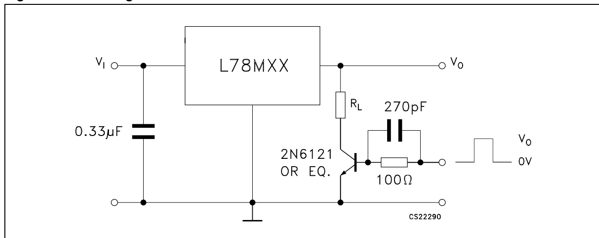
Figure 6. Load regulation
