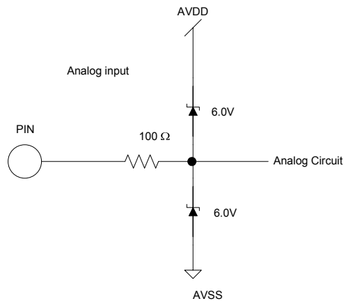
Figure 21 Analog input
