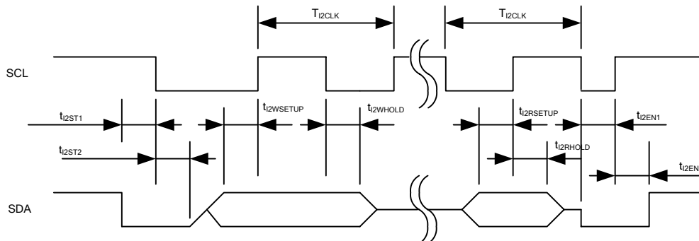
Figure 12 I 2 C AC Timing
