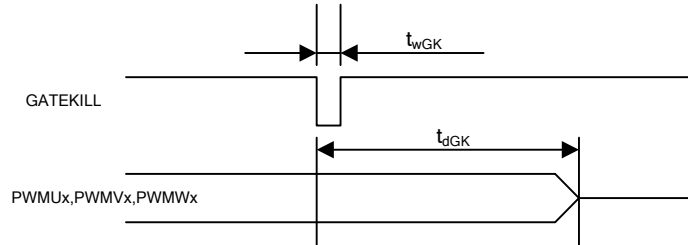
Figure 8. Fault timing
