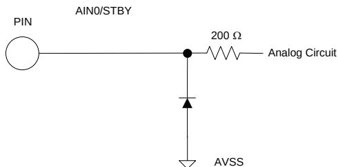
Figure 16 Analog Analog Input Structure for AIN0/STBY
