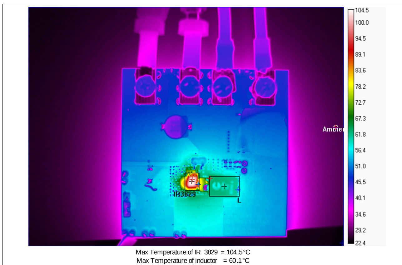
Figure 7-15 Thermal Image of the Board at 16A Load
