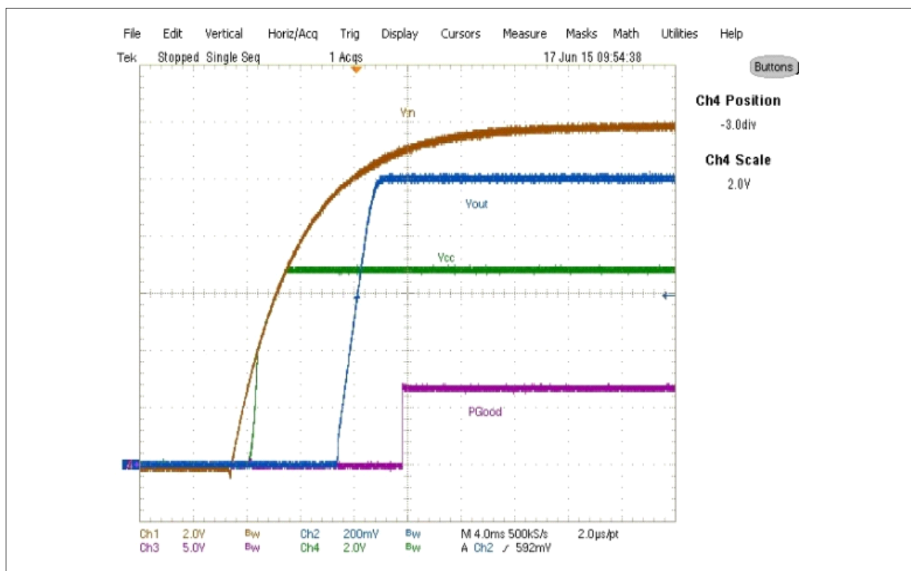
Figure 7-8 Startup at 16A Load (Ch 1 :Vin, Ch 2 :Vout, Ch 3 : PGood, Ch 4 :V CC )
