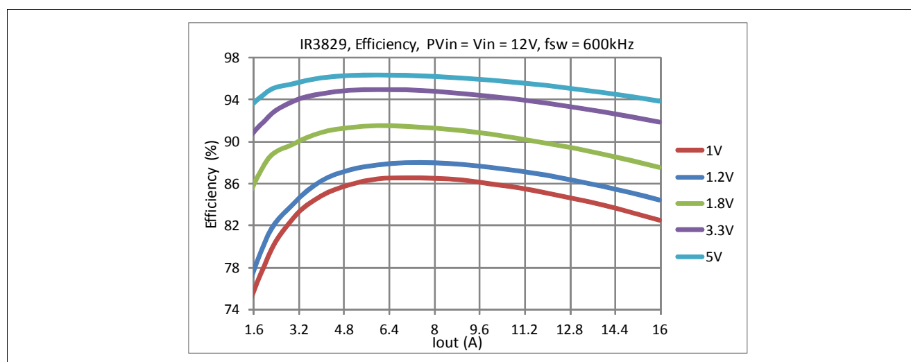
Figure 5-1 IR3829 Efficiency Curves - PV_{in} = V_{in} = 12V , V_{CC} = \text{Internal LDO}
