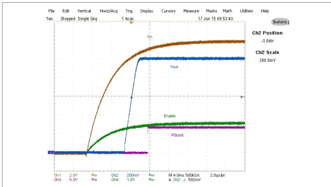
Figure 7-7 Startup at 16A Load (Ch 1 :Vin, Ch 2 :Vout, Ch 3 : PGood, Ch 4 :Enable)
