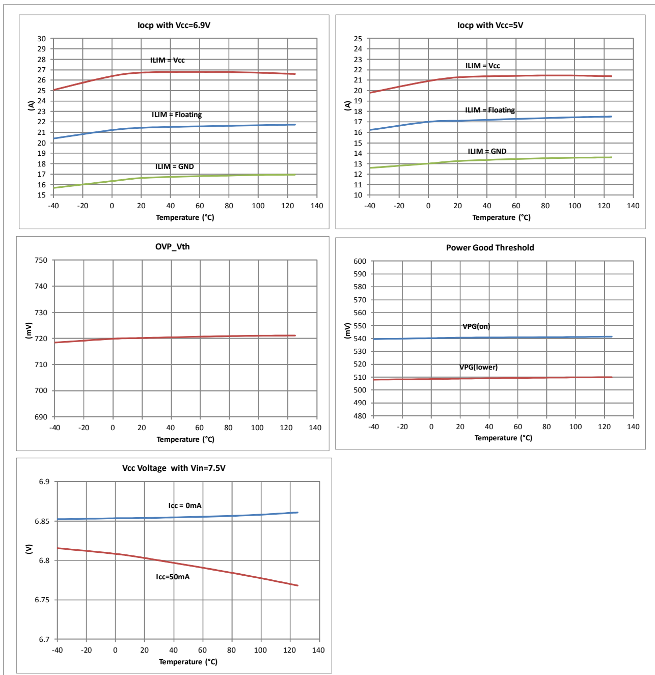
Figure 5-8 Typical Operation Characteristics (Set 2 of 2)
