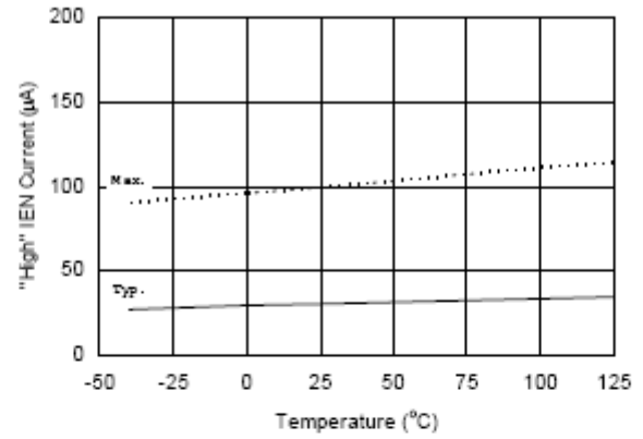
Figure 33A. "High" IEN Current vs. Temperature
