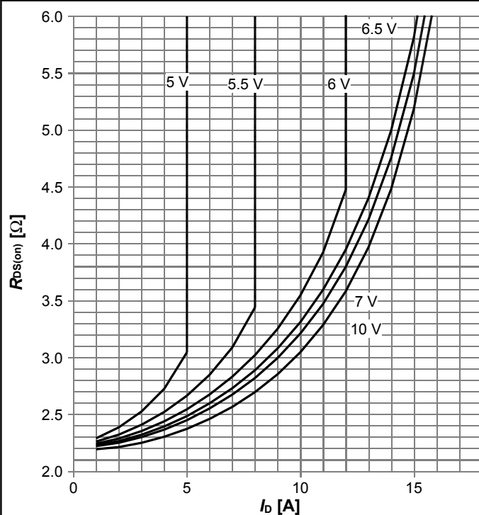
Diagram 7: Typ. drain-source on-state resistance
