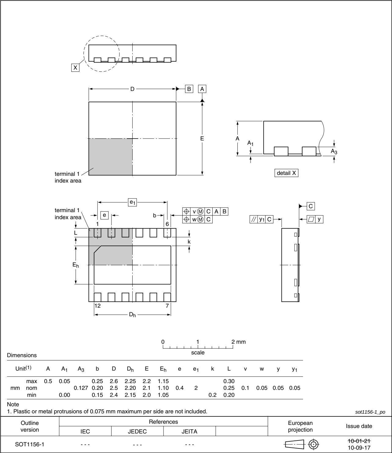
Fig 8. Package outline SOT1156-1 (HXSON12)
