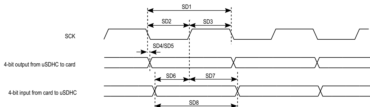
Figure 20. SDR50/SDR104 Timing
