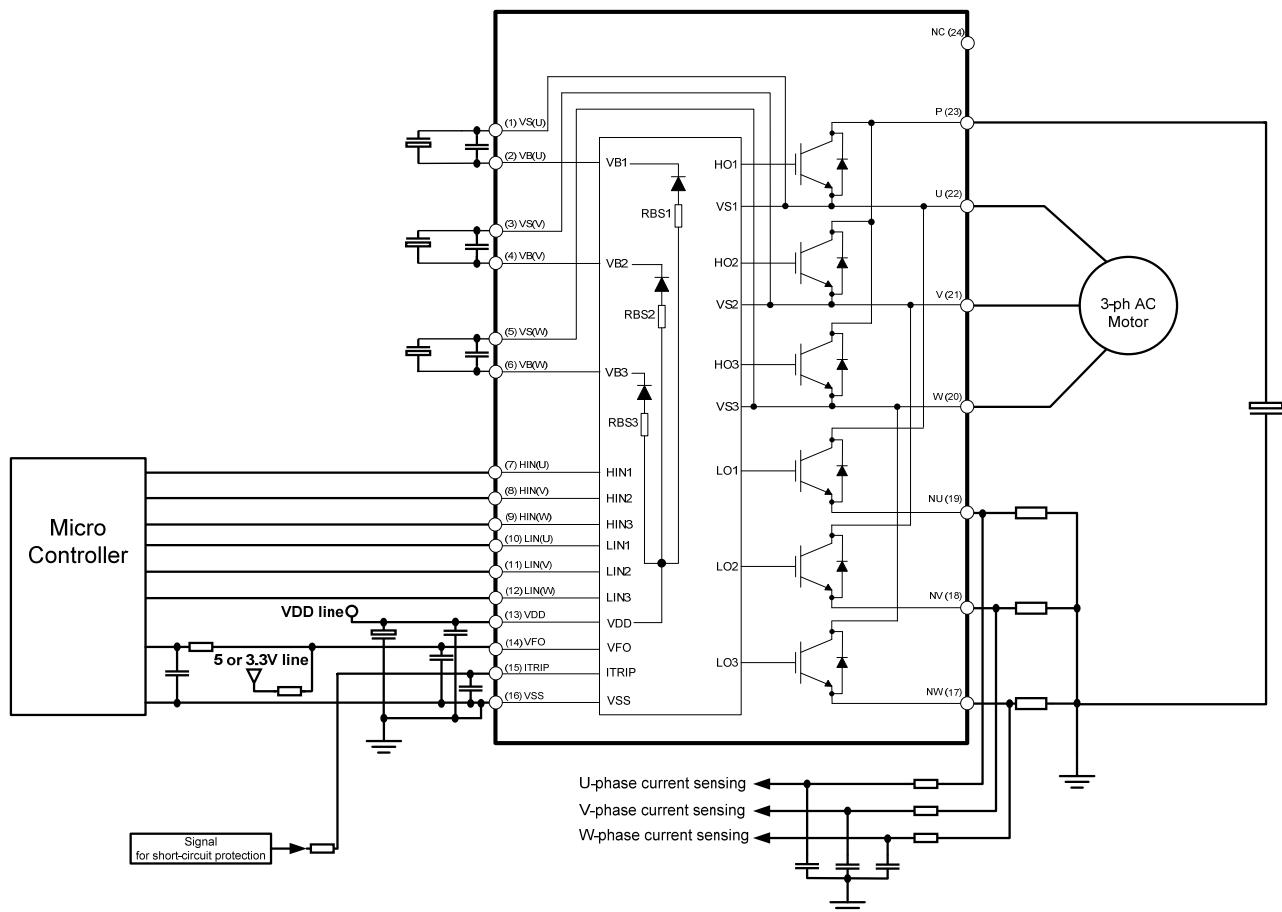
Figure 8: Application circuit
