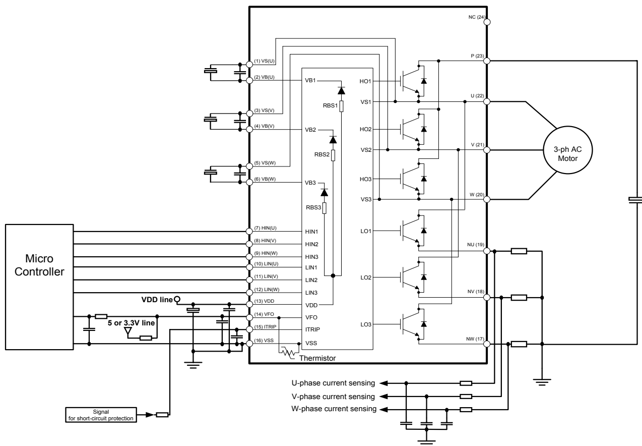
Figure 9: Application circuit
