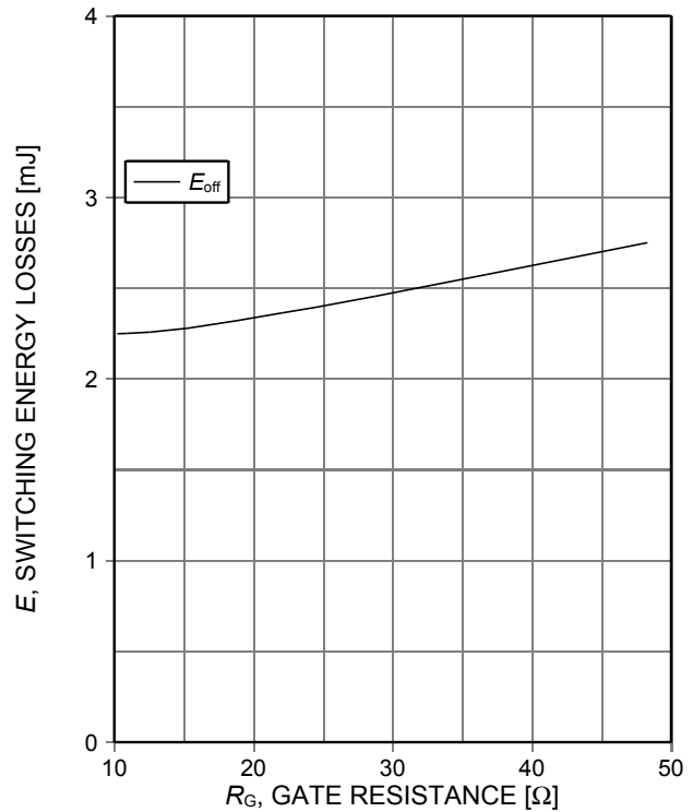
Figure 14. Typical switching energy losses as a function of gate resistance (inductive load, T_{vj}=175^{\circ}\text{C} , V_{CE}=600\text{V} , V_{GE}=0/15\text{V} , I_C=20\text{A} , dynamic test circuit in Figure E)
