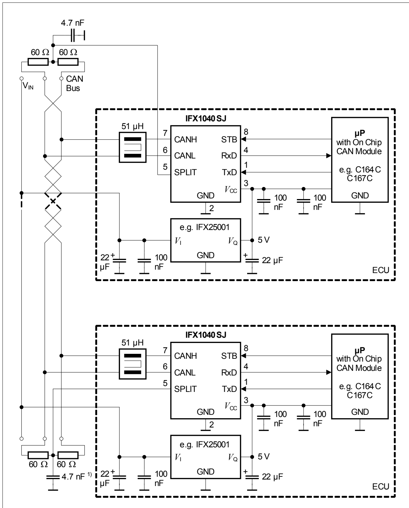
Figure 10 Application Circuit
