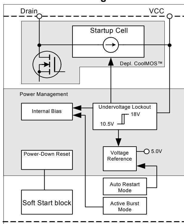
Figure 3 Power Management
