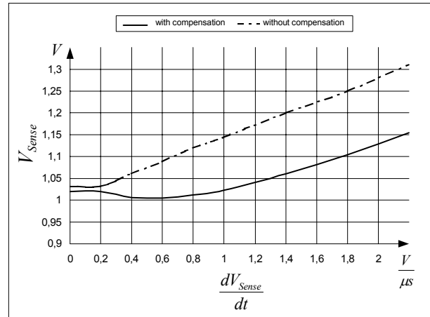
Figure 20 Overcurrent Shutdown
