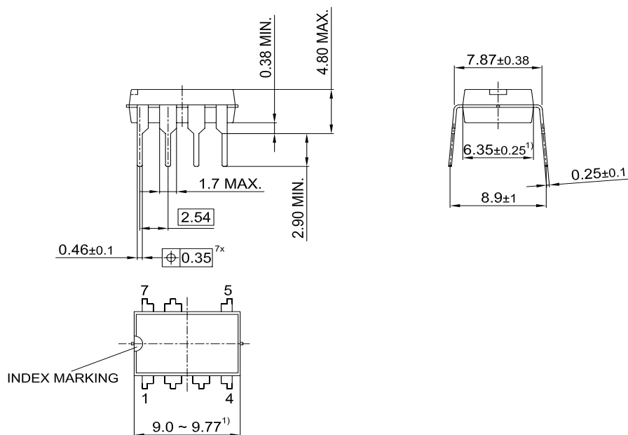
Figure 33 PG-DIP-7 (Pb-free lead plating Plastic Dual-in-Line Outline)
