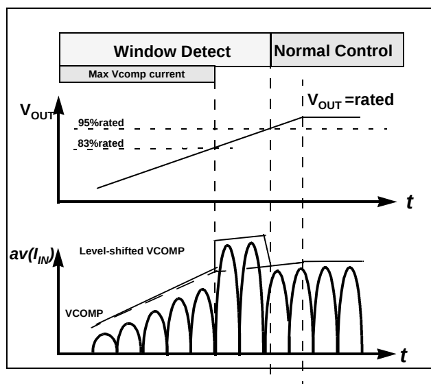
Figure 5 Startup with controlled maximum current
